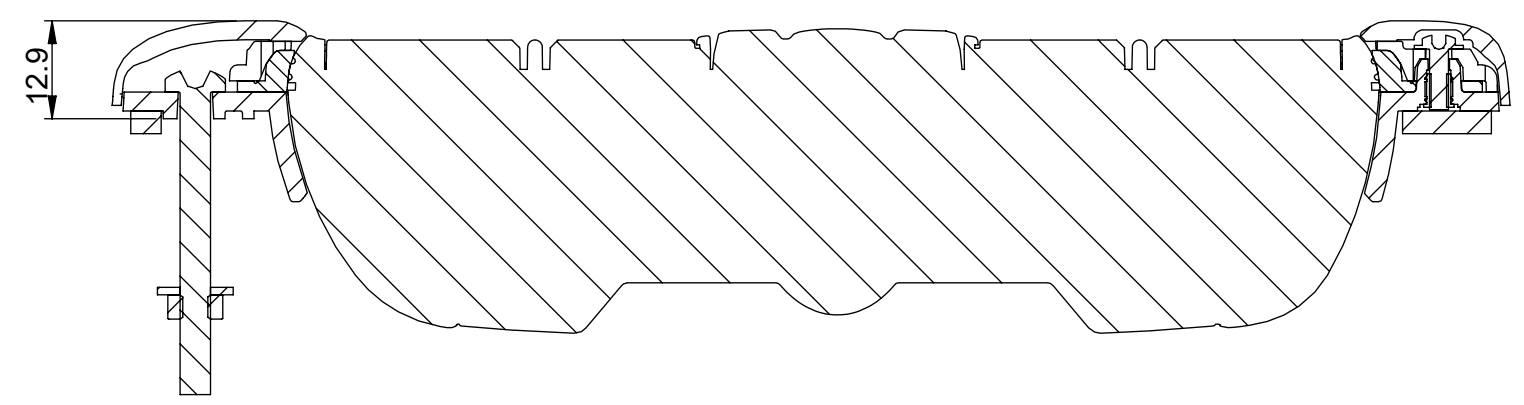
TYPICAL SECTION THROUGH CLAMP PLATE FIXTURE (12 POSITIONS)
